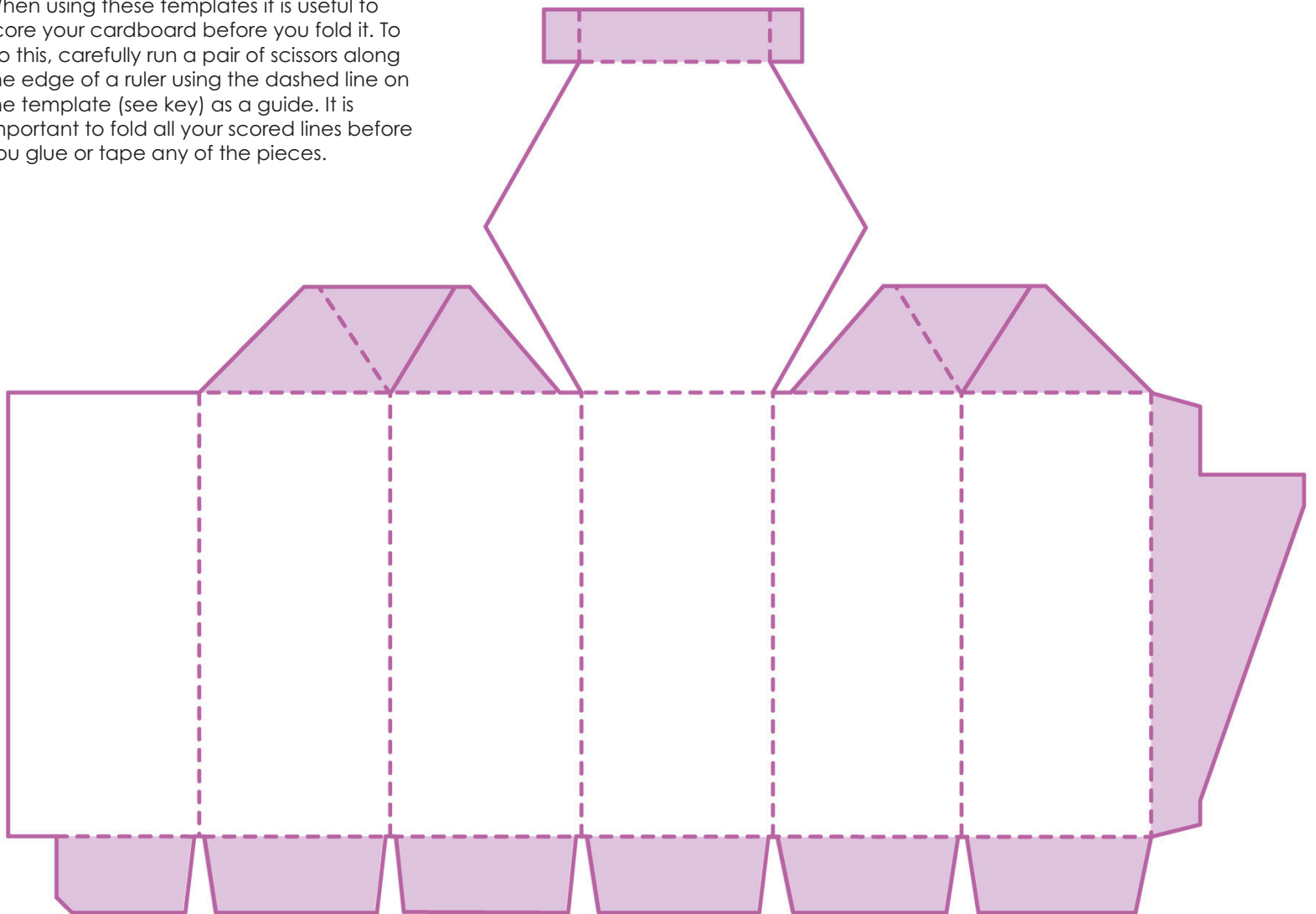
Hexagonal prism: One net template makes one shape.
