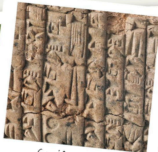
Cuneiform writing
