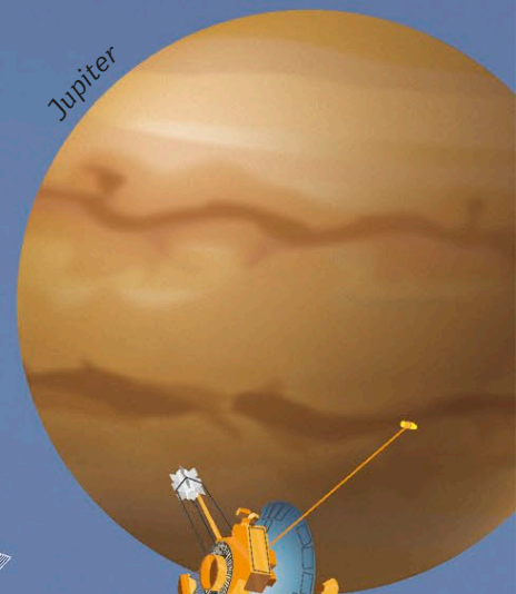
Pioneer 10
