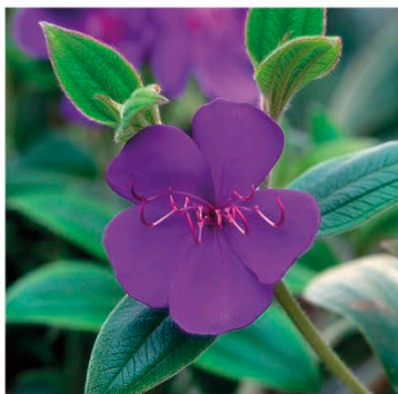
Tibouchina urvilleana (Glory bush)
