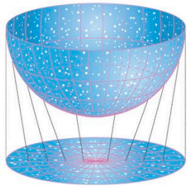
Imagine the Earth surrounded by a sphere of stars. The southern sky map is taken from the bottom half of that sphere.
