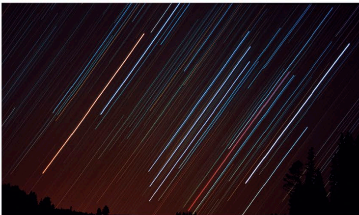
The stars' apparent movement shows clearly on a long exposure photograph of the night sky.
