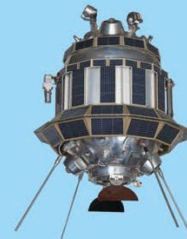
Luna 3
