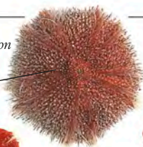
Slate-pencil sea urchin
