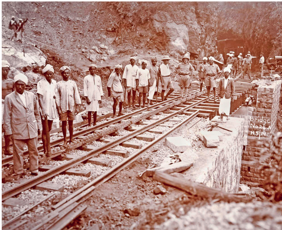
Labourers from the Nilgiri Mountain Railway pause to take a picture with their supervisors next to the railway line. The rack system can be clearly seen in the centre.
