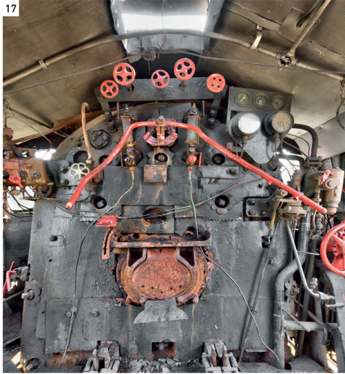
17. Interior of engineer's cab 18. Lubricator box 19. From left to right: injector steam cock handle, dynamo cock, main cock, vacuum steam cock, and injector steam cock handle 20. Firehole door 21. Reverser wheel 22. Steam pressure gauge 23. Rocking grate 24. Front of tender
