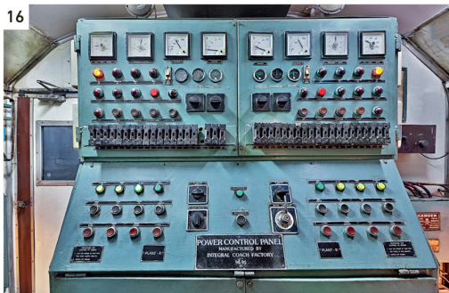
16. Power control panel in the generator car 17. Guard's compartment
