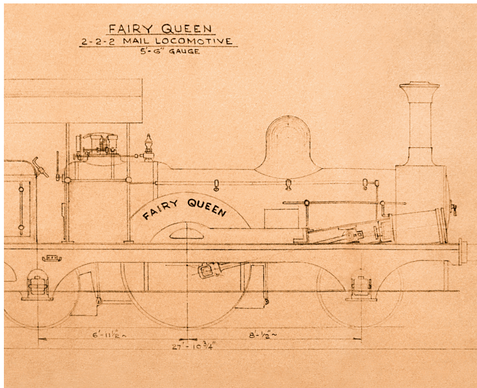
This drawing of the Fairy Queen is a part of the collection in the National Rail Museum in New Delhi, India. The specifics of the engine can be seen mentioned here.
