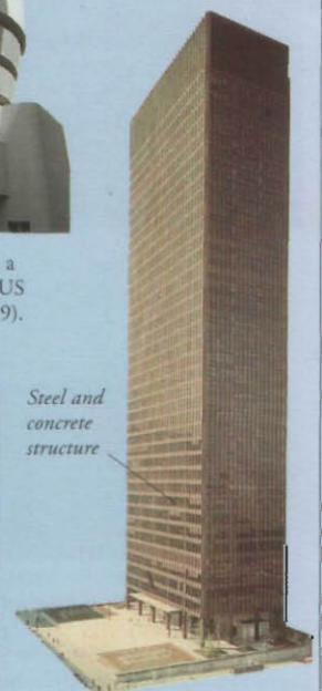
Seagram Building, New York, USA, completed in 1958.
