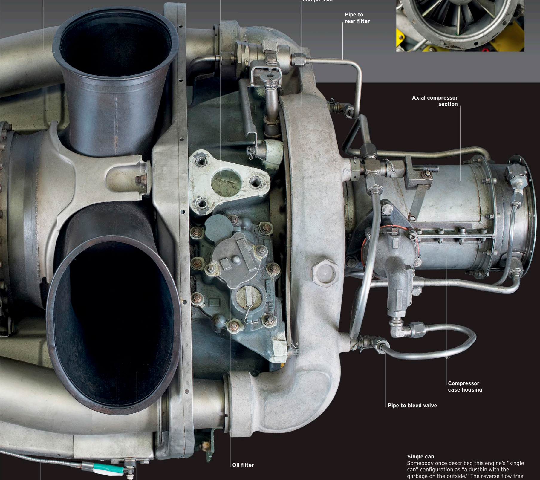
Exhaust outlet Generally located upward in helicopter applications and downward facing in fixed-wing aircraft.
