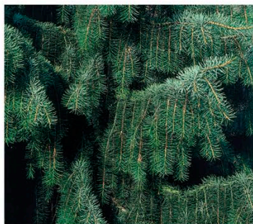
TREE LARGE
