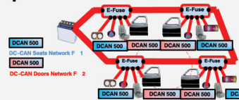
Two CAN Buses share Same Powerline
