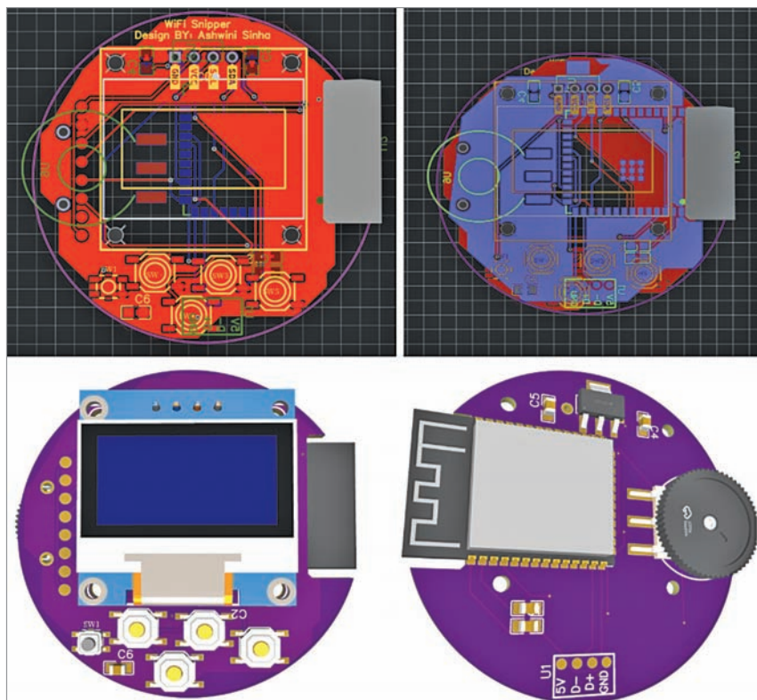
Fig. 3: PCB layout and 3D views
