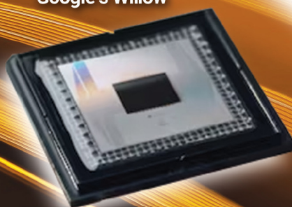
Google's Willow
