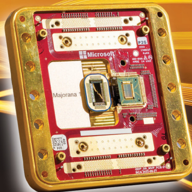
Microsoft's Majorana 1
