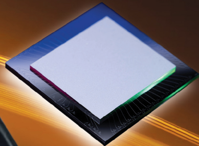
Amazon's Ocelot
