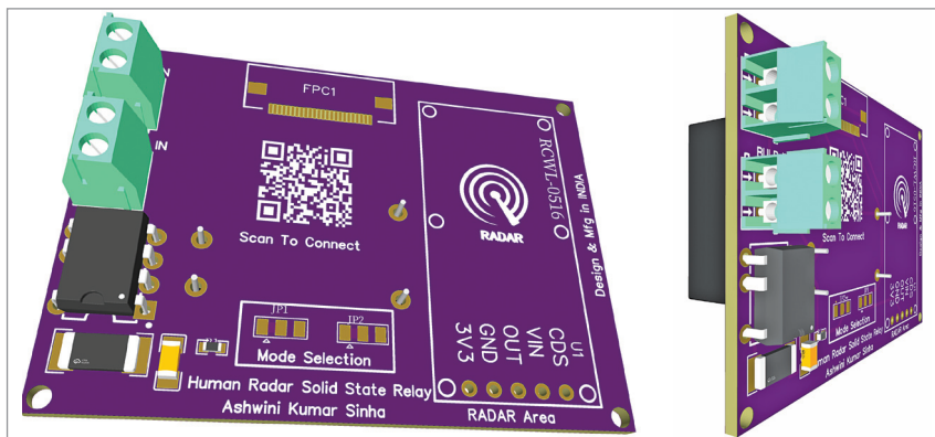
Fig. 1: Author's prototype design
