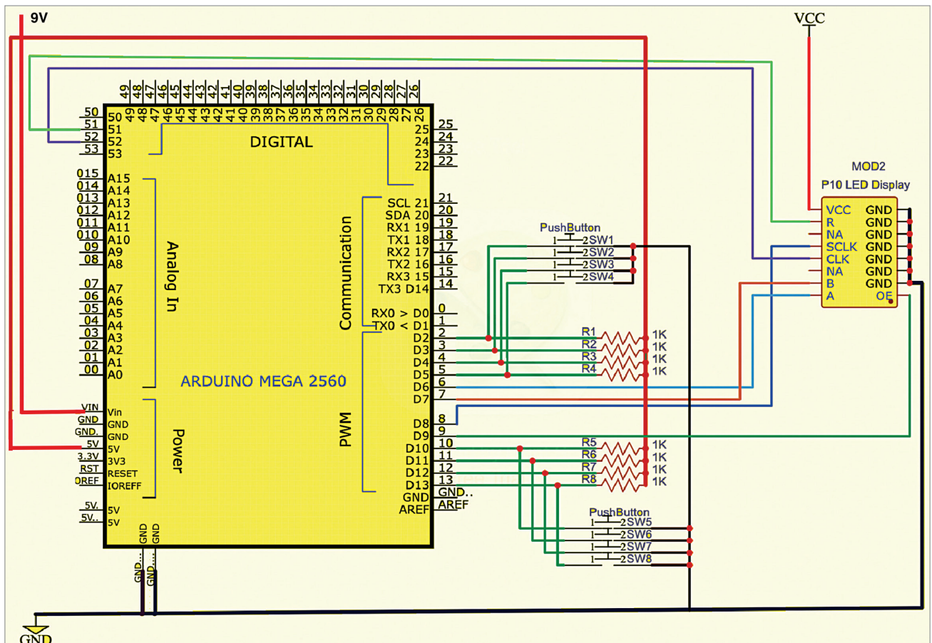
Fig. 2: Circuit diagram
