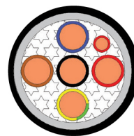
6 Core Charging Cable
