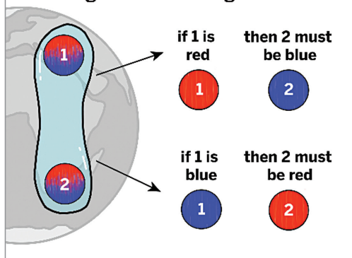
Fig. 3: Quantum entanglement (Source: https://quantumatlas.umd.edu )
