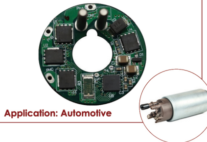
BLDC CONTROLLER- FUEL PUMP
