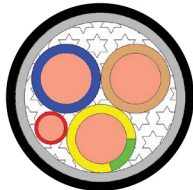
4 Core Charging Cable
