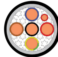
6 Core Charging Cable
