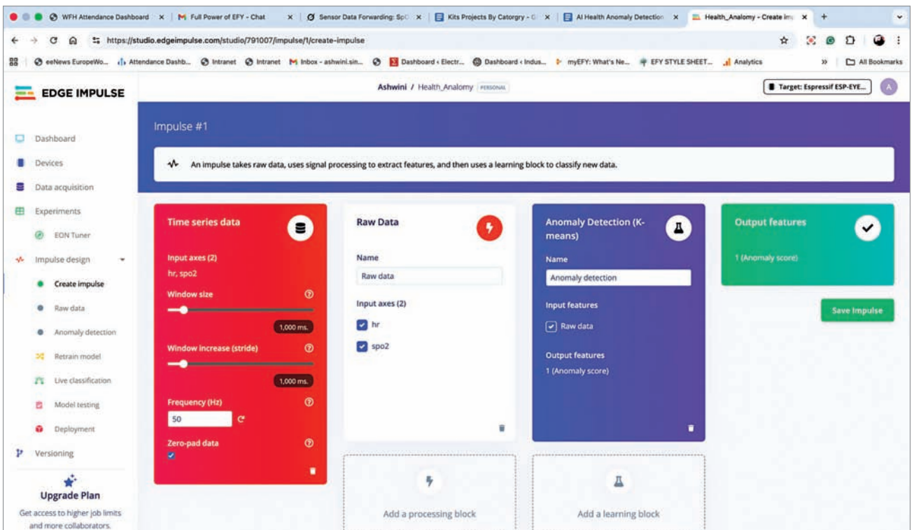
Fig. 4: Impulse design section of Edge Impulse
