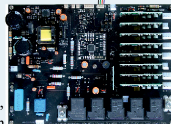
QUIKorrect 200KVA PCB
