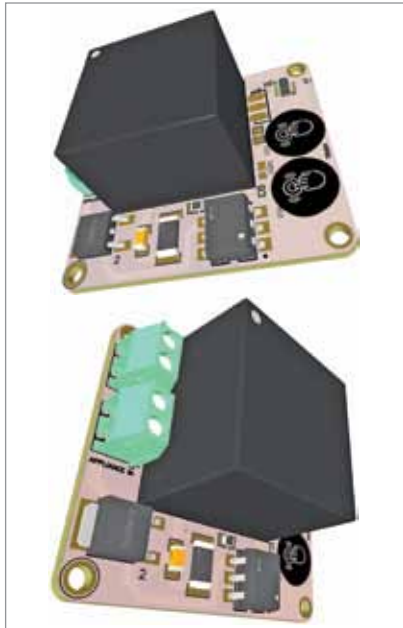
Fig. 1: Touch solid-state relay (SSR) PCB
