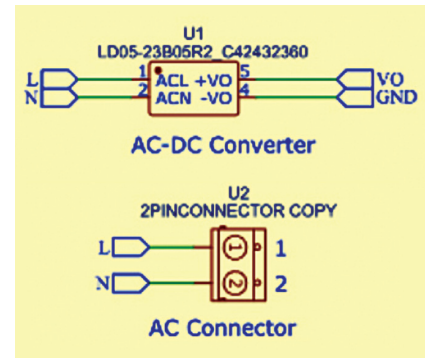
Fig. 2: Circuit diagram of AC-DC converter
