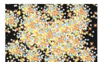
㉓ the universe
