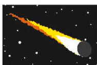
⑳ meteor
