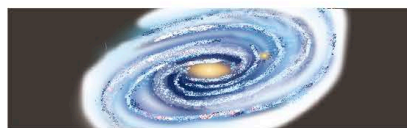
㉒ the Milky Way
