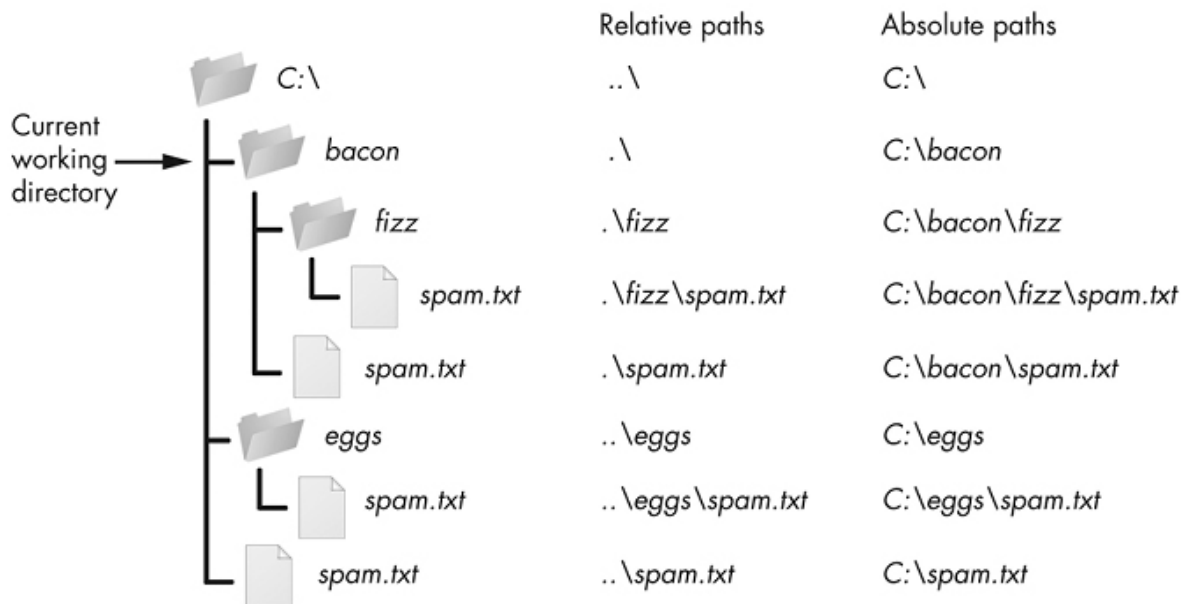
Figure 2-2: The relative paths for folders and files in the working directory C:\bacon
