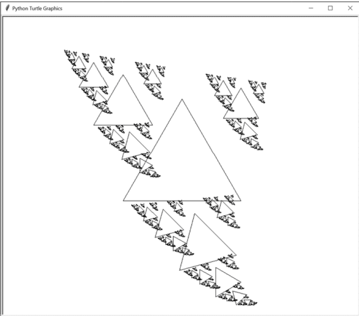
Figure 13-5: The final Wave fractal after each triangle recursively generates three more triangles
