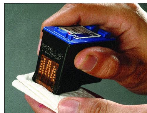
Place the cartridge as shown above to clean the nozzle
