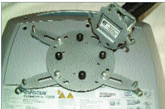
Align the screws of the ceiling mount exactly with the drilled holes at the back of the projector
