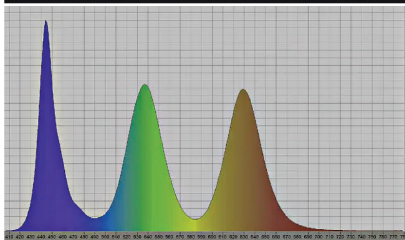
Distinct Red, Green and Blue Waveforms in Samsung QLED TV
