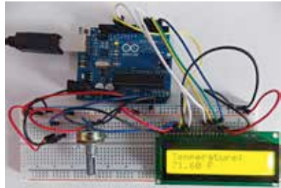
Hardware to sense current temperature
