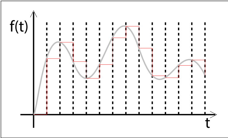
A step response that hasn't been smoothed out after DAC
