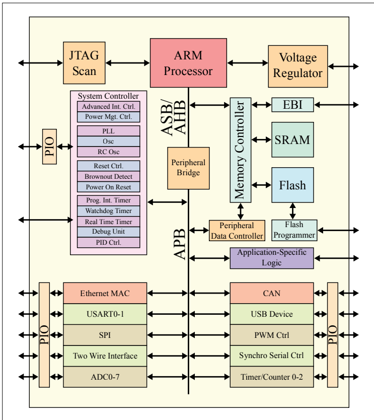
Generic ARM SoC Block diagram
