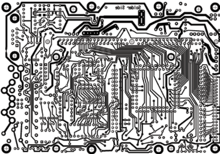
A PCB Layout
