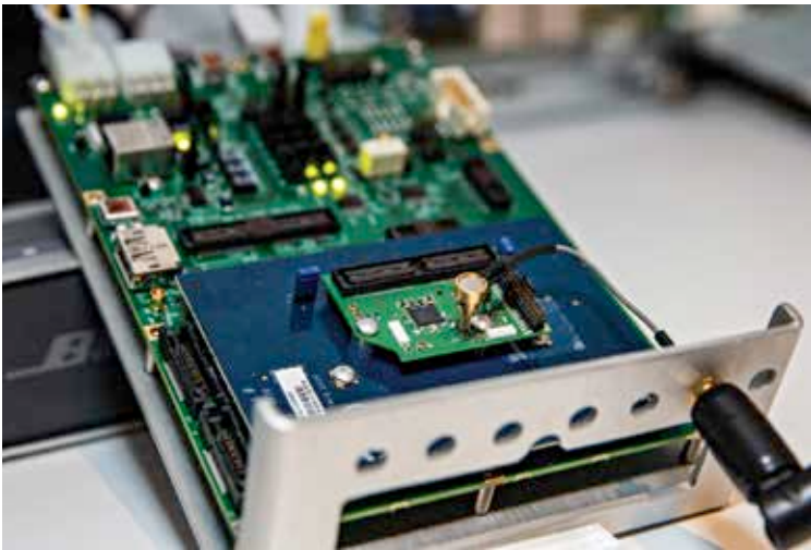
Intel's Lightning Peak Chipset On Display.
