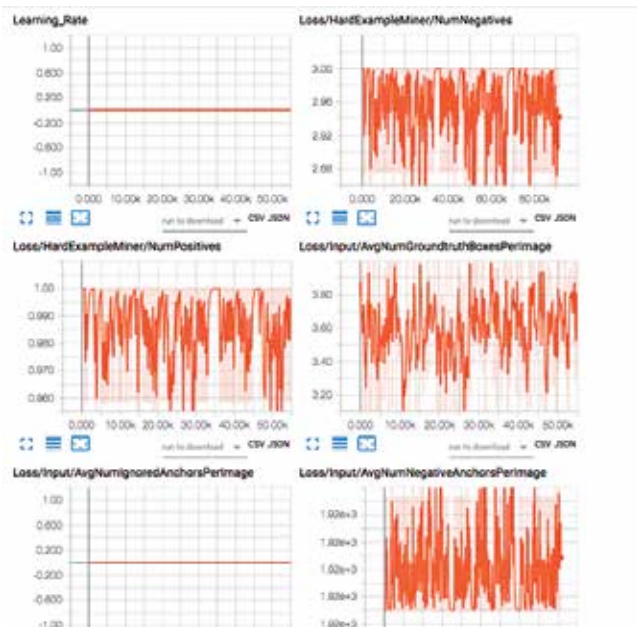
Loss Function Graphs Generate From Code
