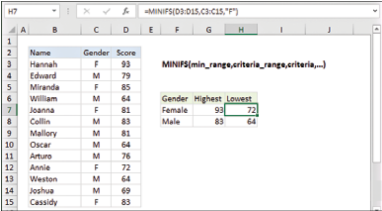
How MINIFS works
