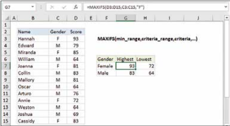
How MAXIFS works
