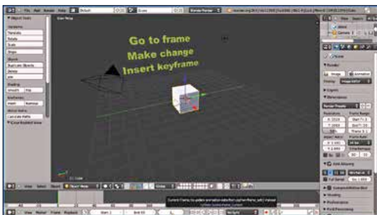
Inserting keyframes
