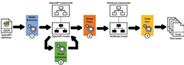
REST API FlowChart
