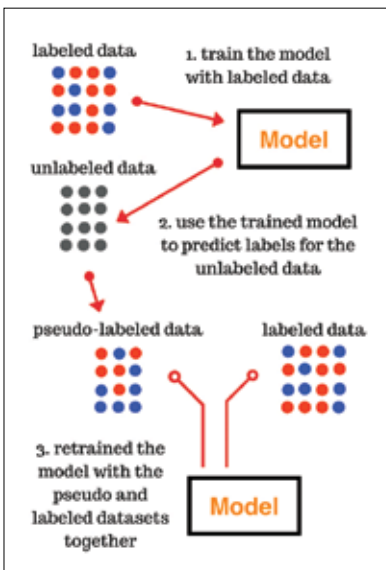
Semi-supervised Model
