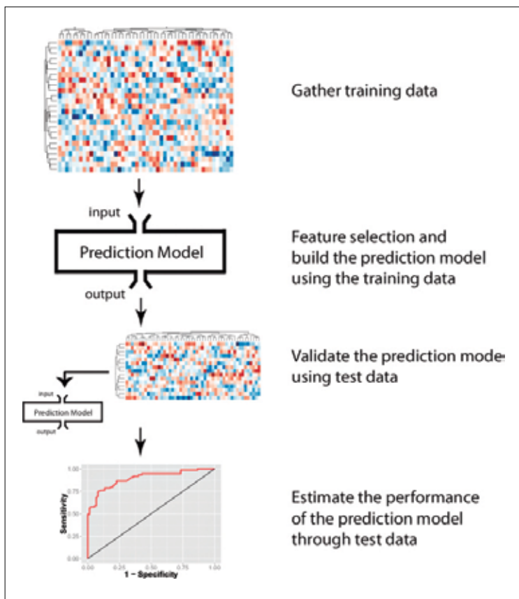
Testing Dataset
